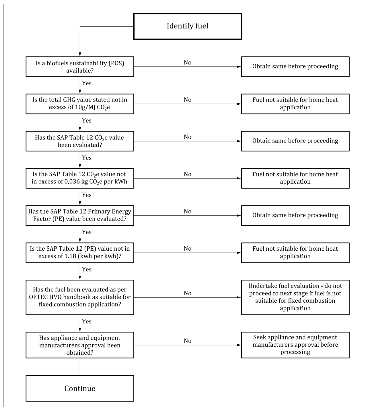
Figure 1 – Fuel evaluation process flowchart
